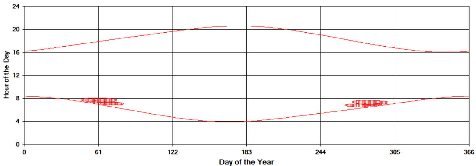
Shadow Times on House 26, All Windows from All Turbines
