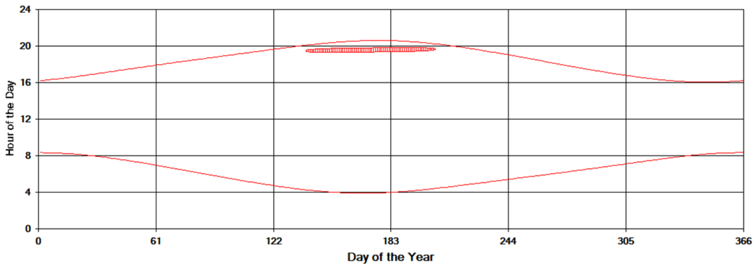
Shadow Times on House 19, All Windows from All Turbines
