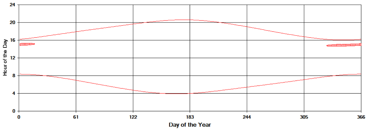
Shadow Times on House 29, All Windows from All Turbines
