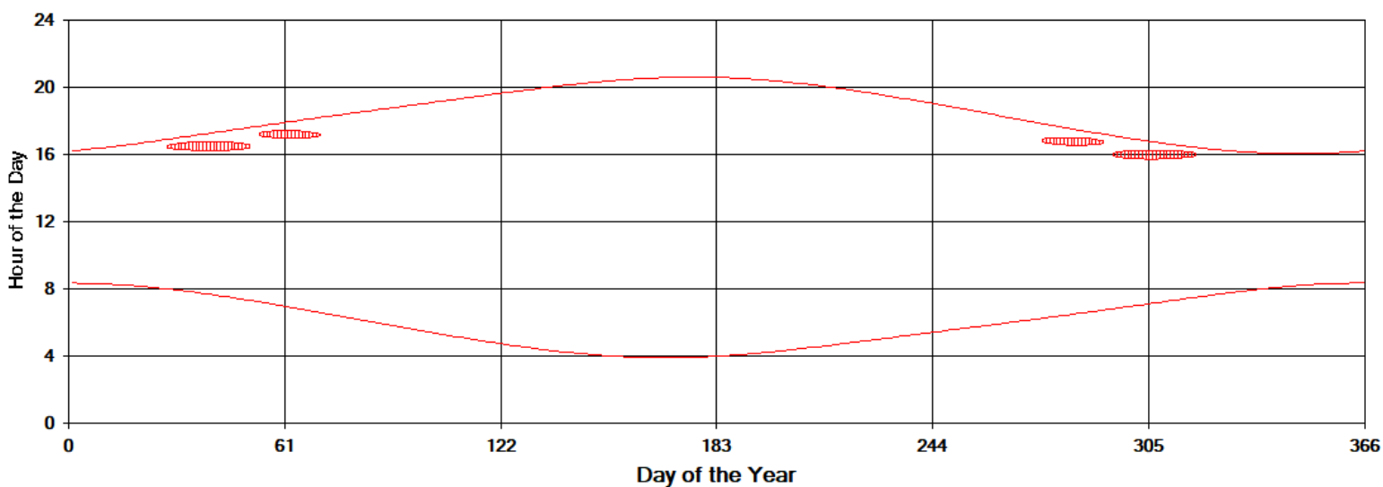
Shadow Times on House 18, All Windows from All Turbines
