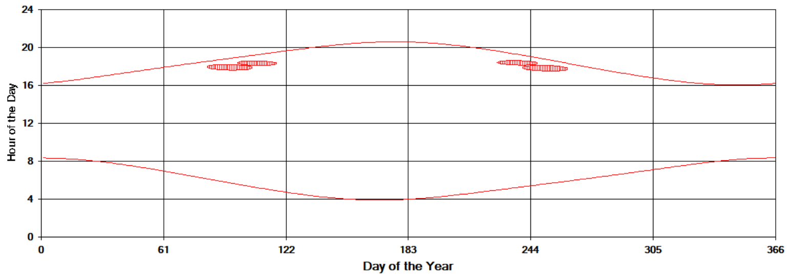
Shadow Times on House 10, All Windows from All Turbines
