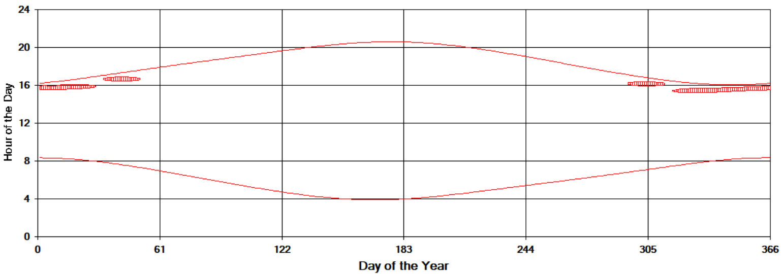
Shadow Times on House 24, All Windows from All Turbines
