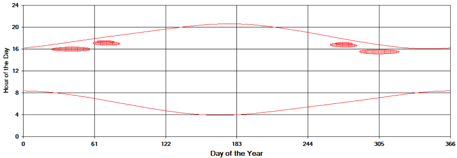
Shadow Times on House 3, All Windows from All Turbines
