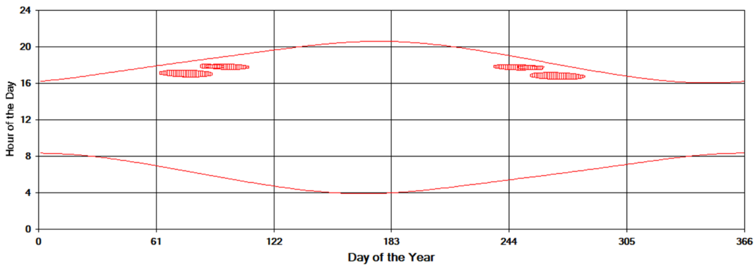
Shadow Times on House 6, All Windows from All Turbines
