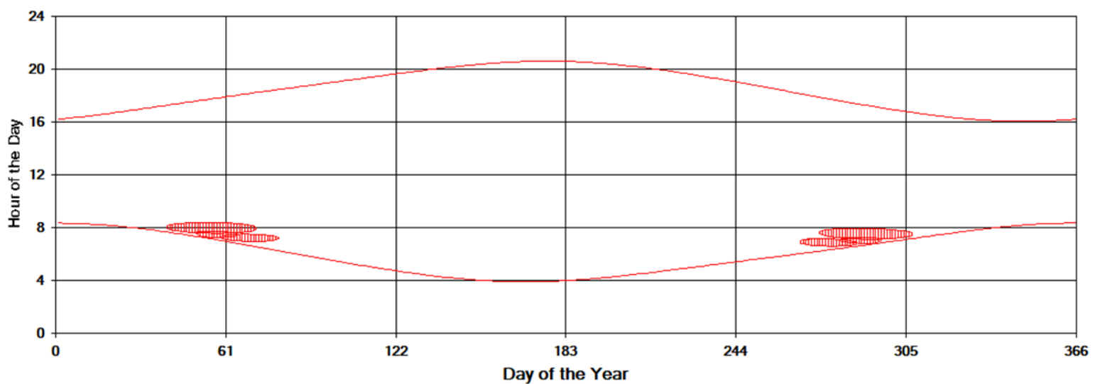
Shadow Times on House 27, All Windows from All Turbines
