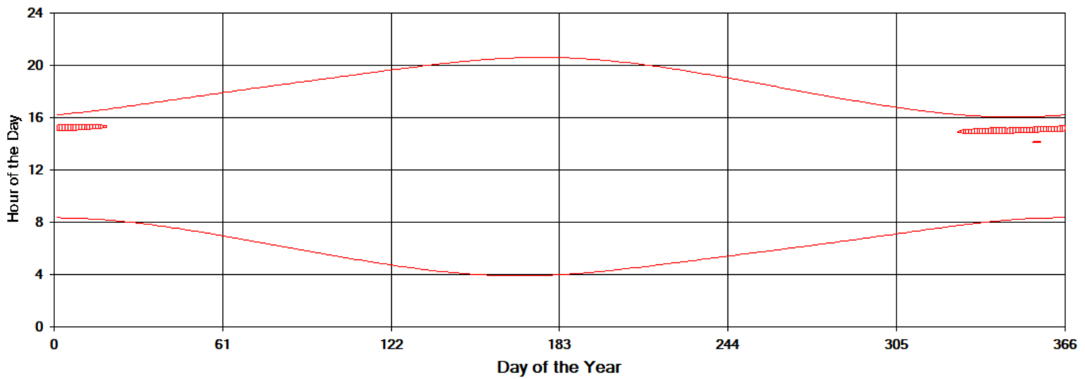
Shadow Times on House 35, All Windows from All Turbines
