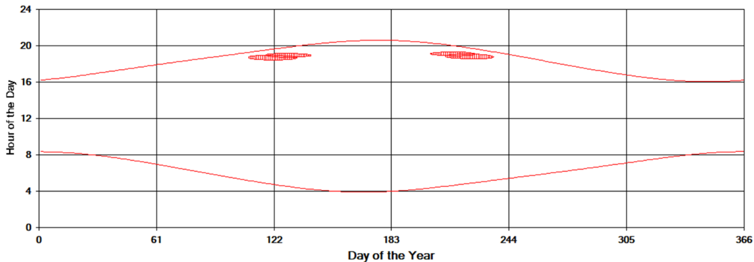
Shadow Times on House 25, All Windows from All Turbines
