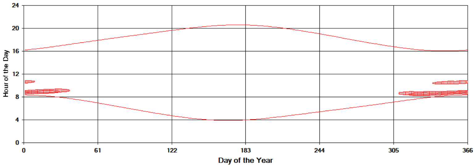
Shadow Times on House 28, All Windows from All Turbines
