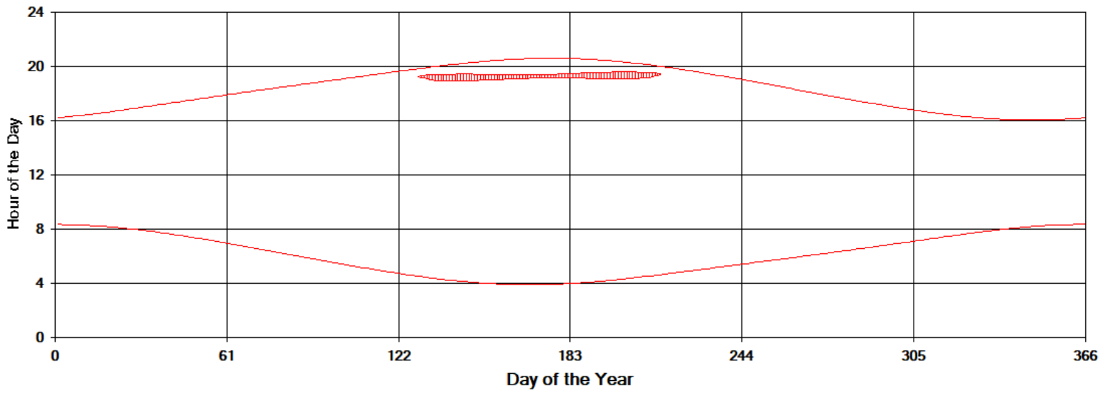
Shadow Times on House 1, All Windows from All Turbines
