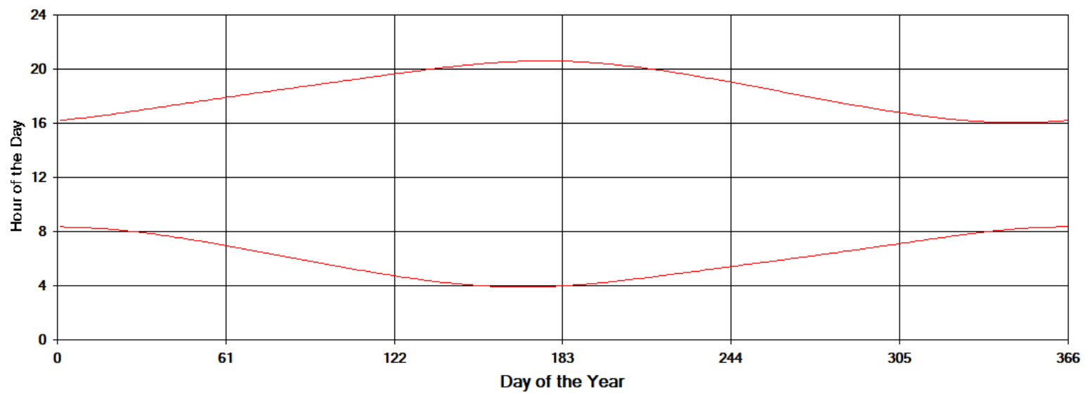
Shadow Times on House 43, All Windows from All Turbines
