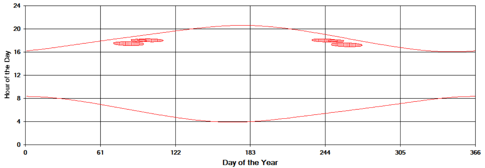
Shadow Times on House 8, All Windows from All Turbines
