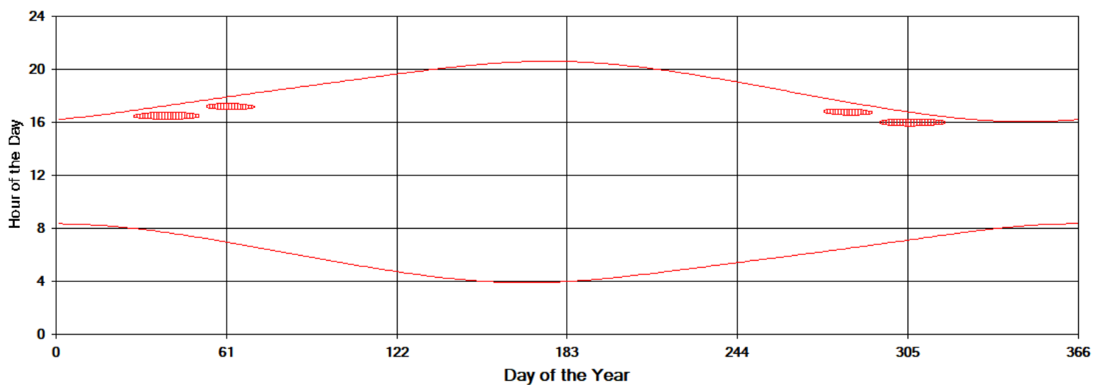
Shadow Times on House 17, All Windows from All Turbines
