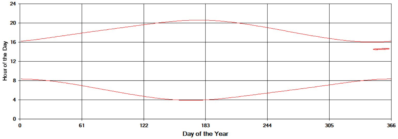
Shadow Times on House 31, All Windows from All Turbines
