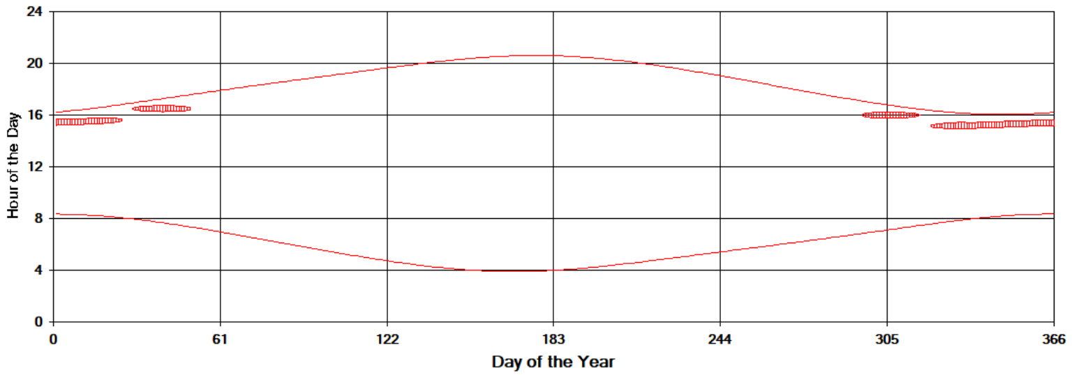
Shadow Times on House 22, All Windows from All Turbines
