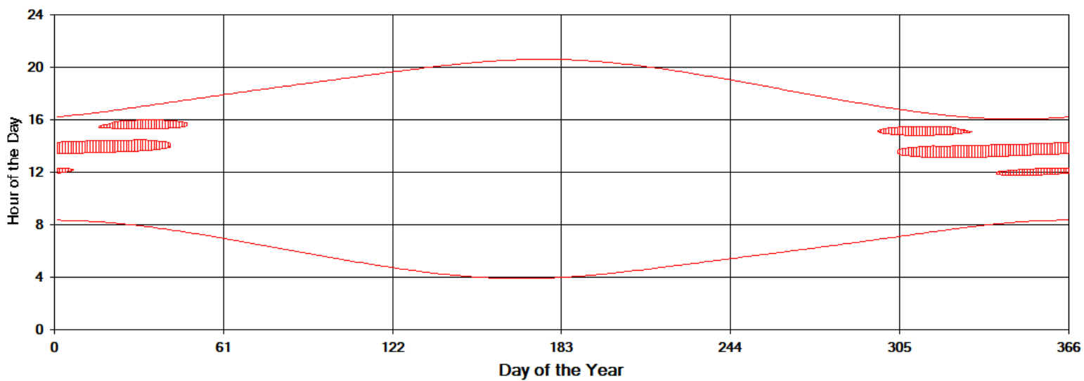
Shadow Times on House 36, All Windows from All Turbines
