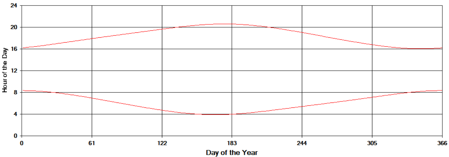
Shadow Times on House 33, All Windows from All Turbines
