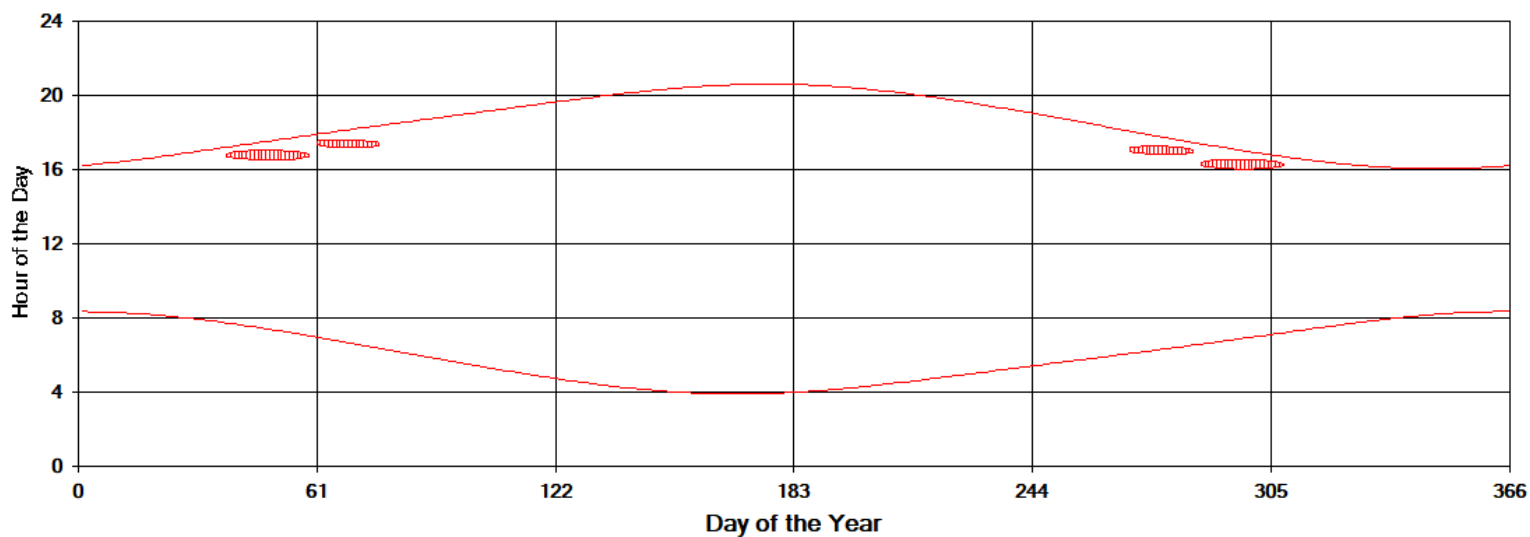
Shadow Times on House 16, All Windows from All Turbines
