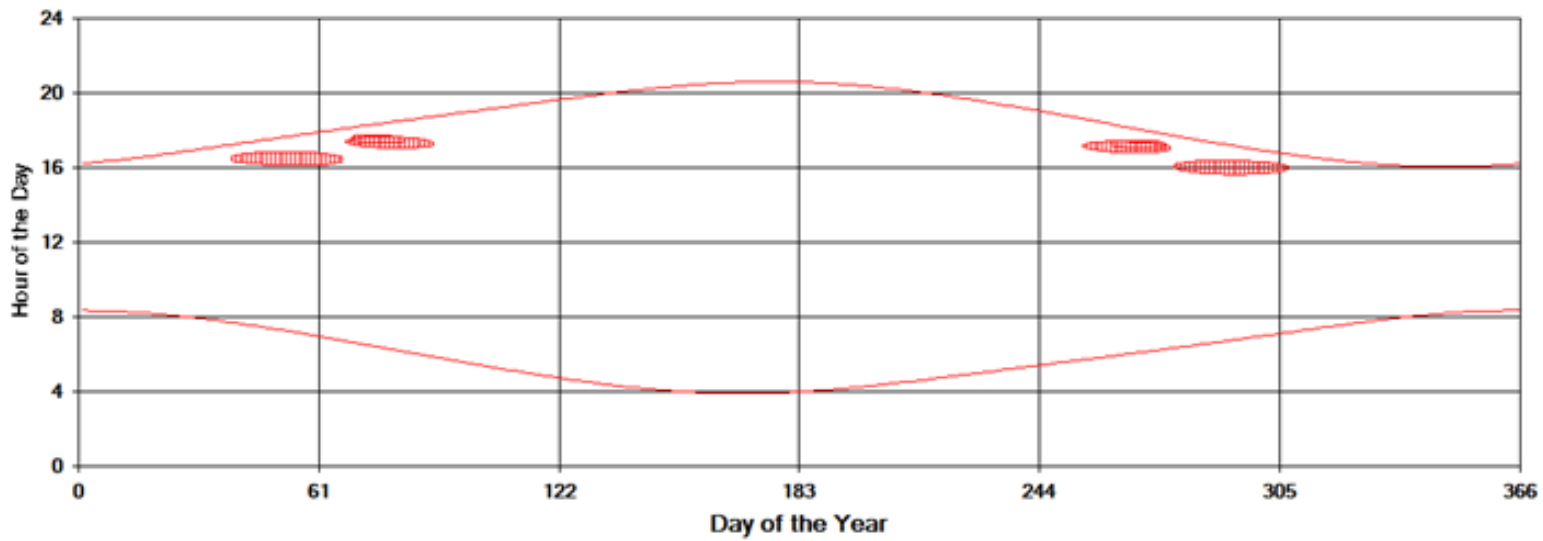
Shadow Times on House 5, All Windows from All Turbines
