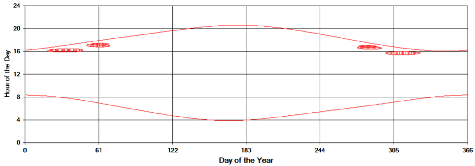
Shadow Times on House 20, All Windows from All Turbines
