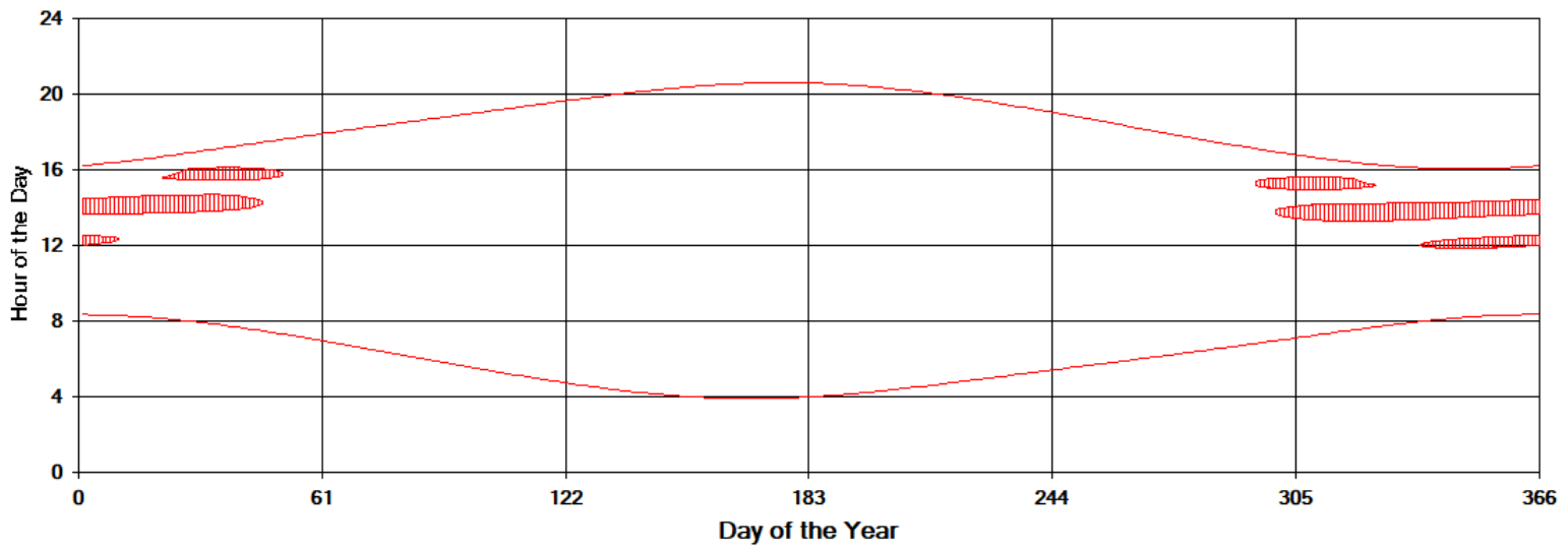
Shadow Times on House 37, All Windows from All Turbines
