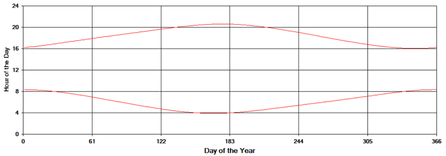
Shadow Times on House 30, All Windows from All Turbines
