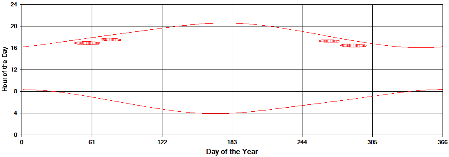
Shadow Times on House 14, All Windows from All Turbines
